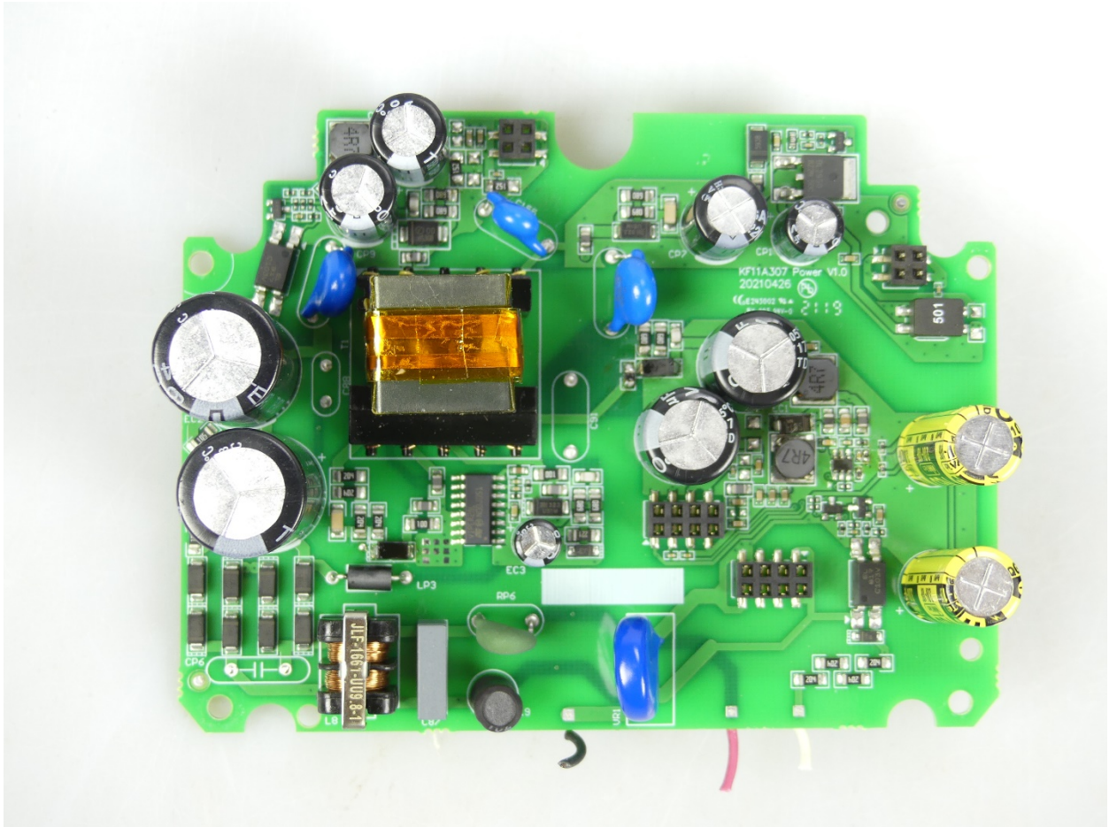
Power PCB version 2
